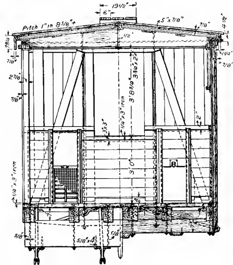
Fig. 266. Cross Sections through Door and Bolster.
